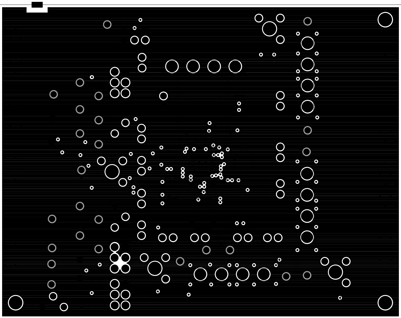
FIGURE 5. L2 GND
